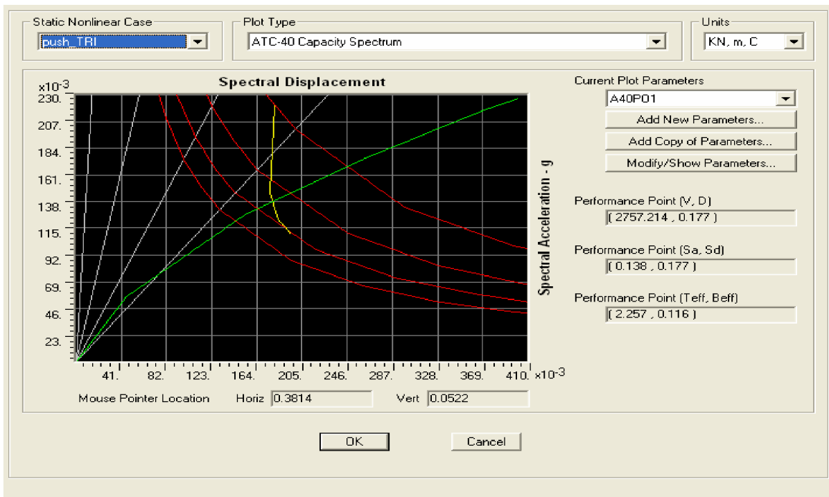
Fig.4.16 Capacity spectrum of eight storey building for Triangular Load Pattern
