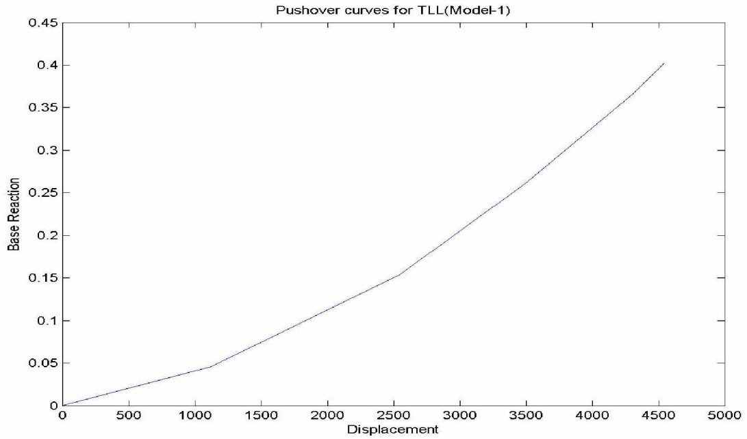
Fig 4.5 Pushover curve for triangular lateral load pattern
