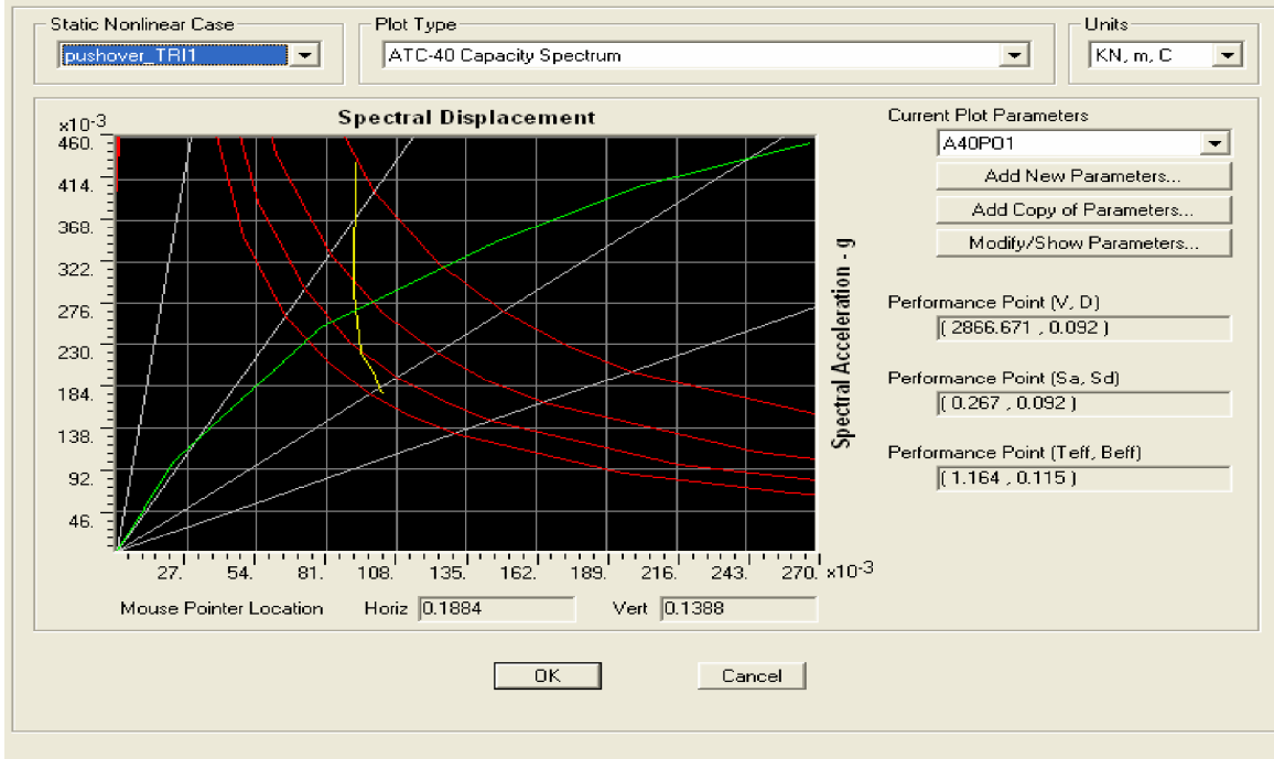
Fig.4.13 Capacity spectrum of four storey building for Triangular Load Pattern.
