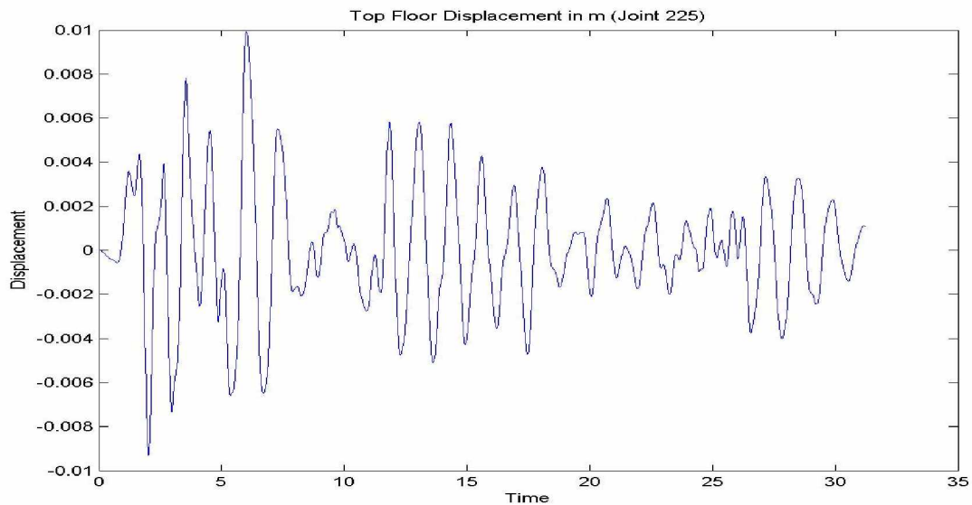
Fig: 4.3 Displacement time history of top floor (shorter direction) – model 2 (peak – 0.009947m)
