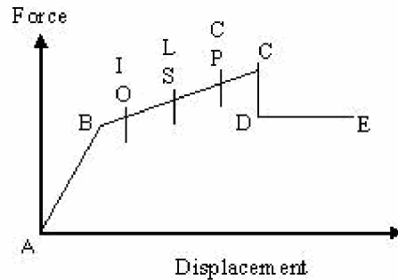
Fig 1.3 Different stages of plastic hinge
