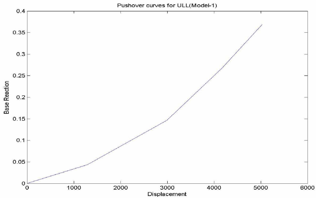
Fig 4.6 Pushover curve for uniform lateral load pattern
