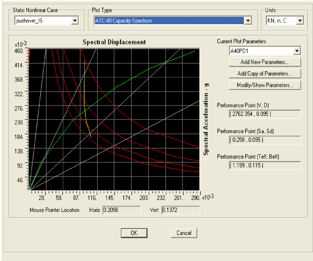
Fig.4.12 Capacity spectrum of four storey building for Parabolic Load Pattern.
