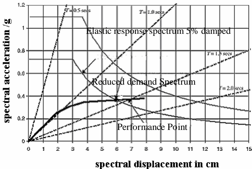
Capacity spectrum
