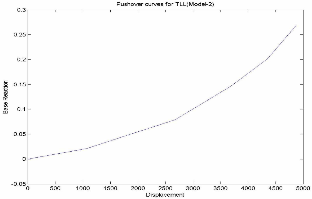
Fig 4.8 Pushover curve for triangular lateral load pattern
