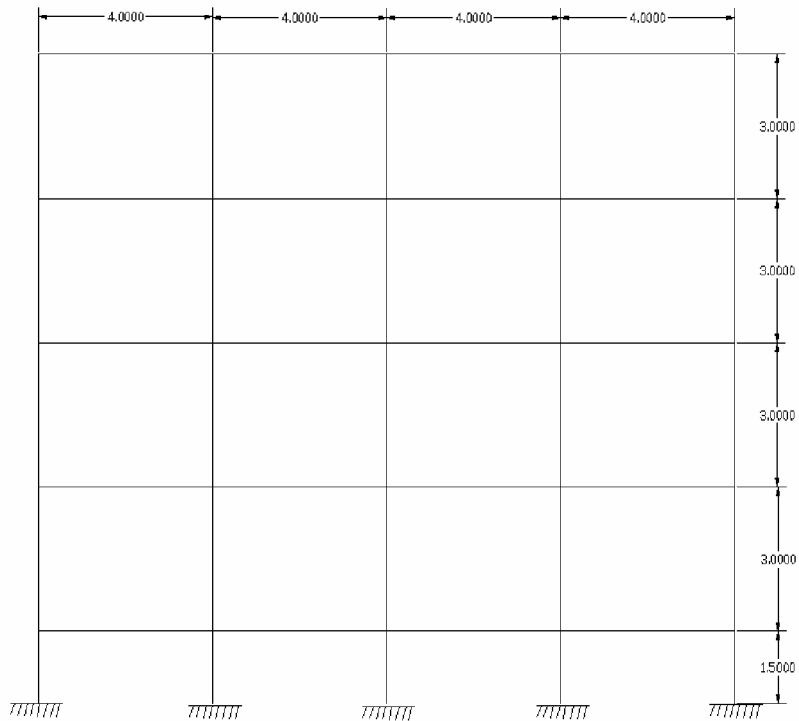
Elevation for four storey(G+4) building
