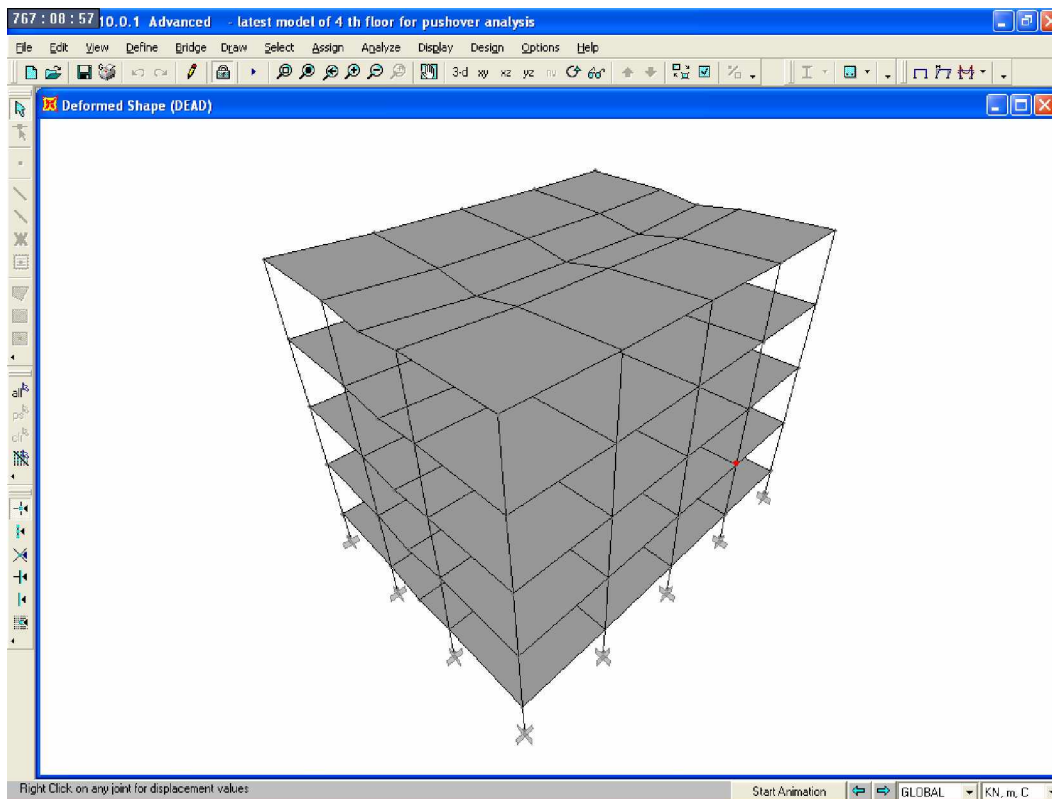
Fig 3.2 3-D view of the four storey (G+4) building created in SAP2000
