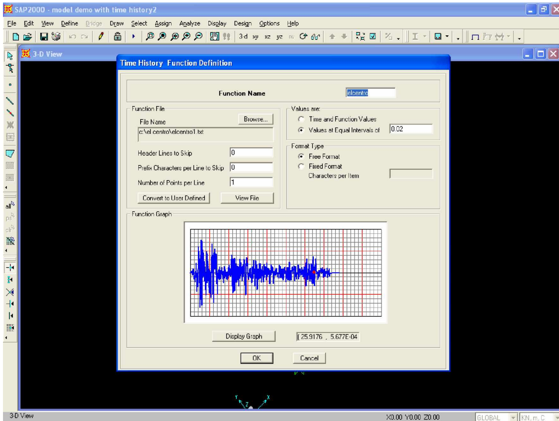
Fig: 3.8 Defining time history function (Elcentro, 1940) in SAP2000
