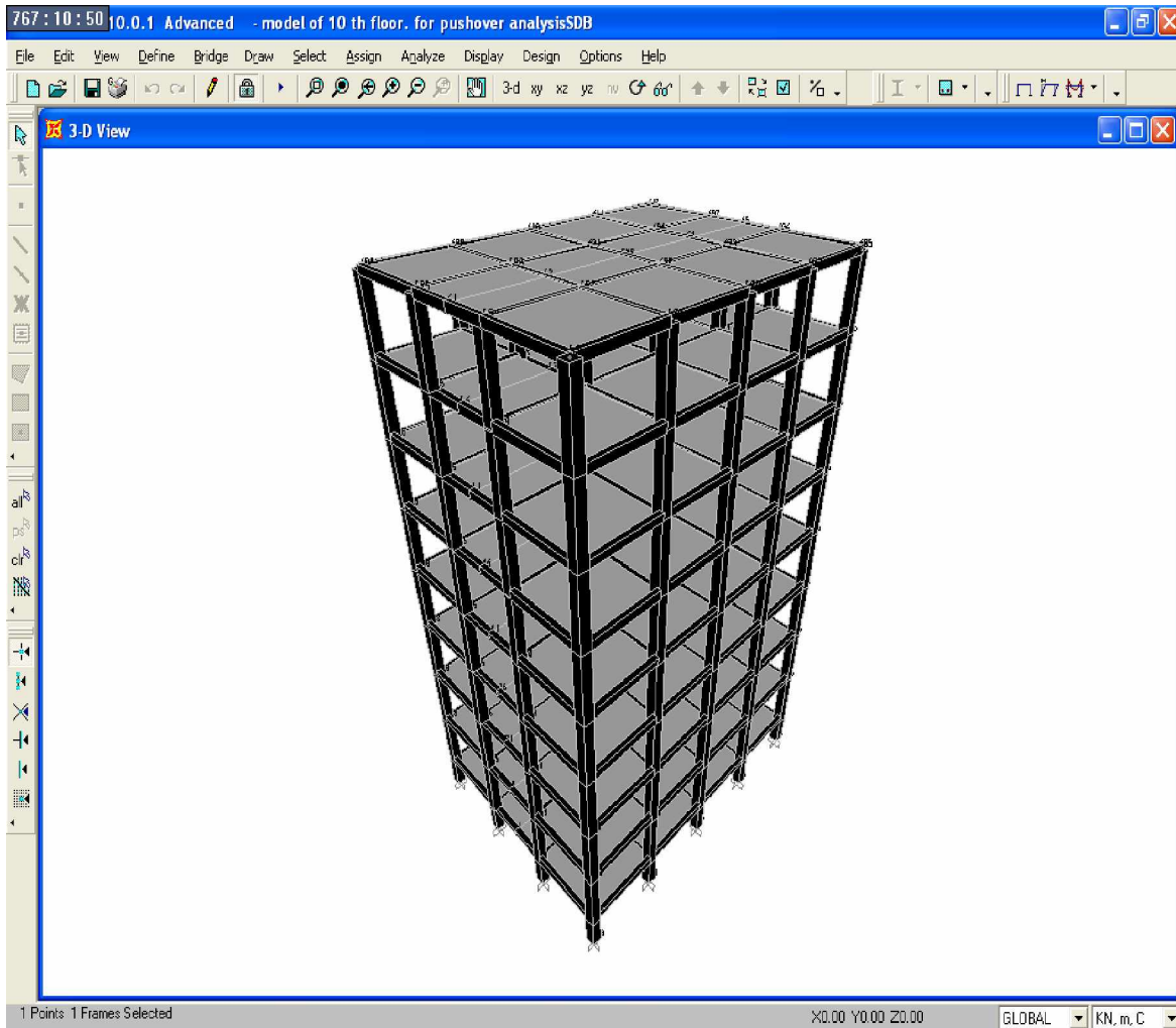
Fig 3.3 3-D view of the eight storey building (G+8) created in SAP2000
