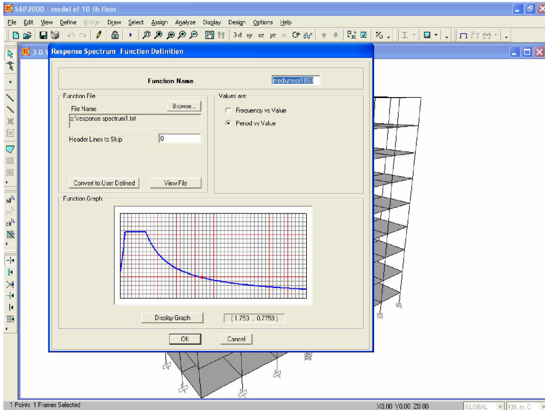
Fig 3.6 Defining response spectrum function ( S_d/g ) Vs. Period (table 3.1) in SAP2000
