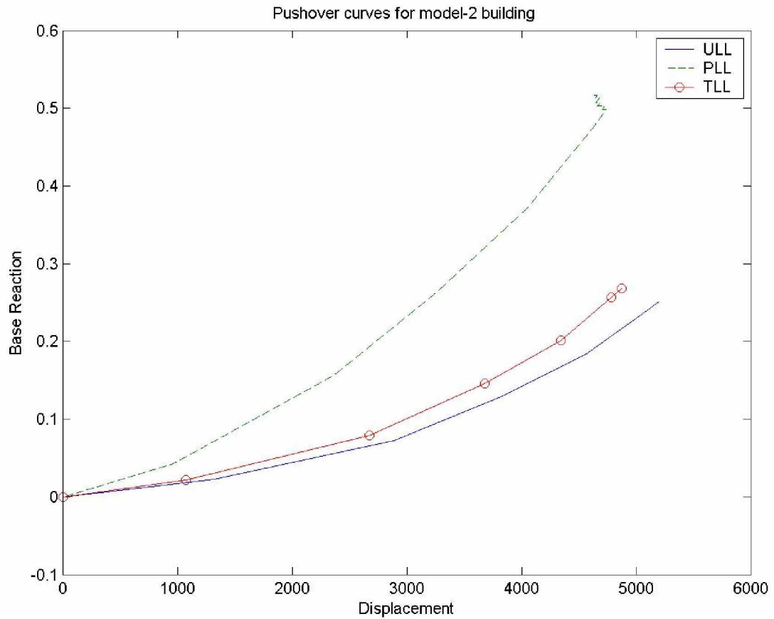
Fig. 4.11 Pushover curves of rigid floor diaphragm for different lateral load patterns of eight storey building.
