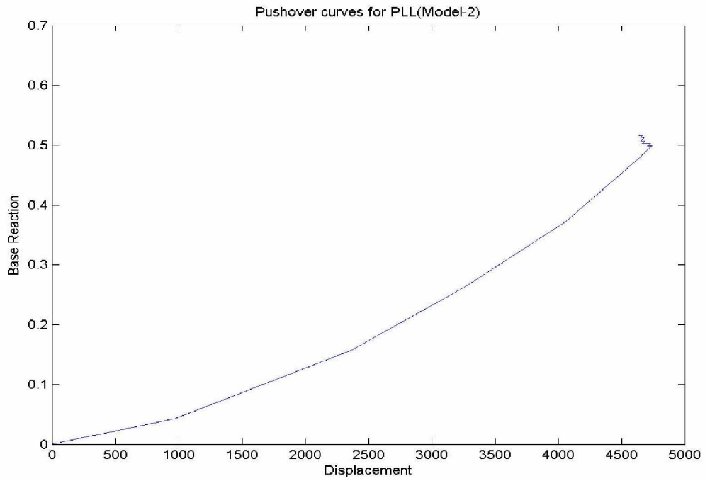
Fig 4.7 Pushover curve for parabolic lateral load pattern
