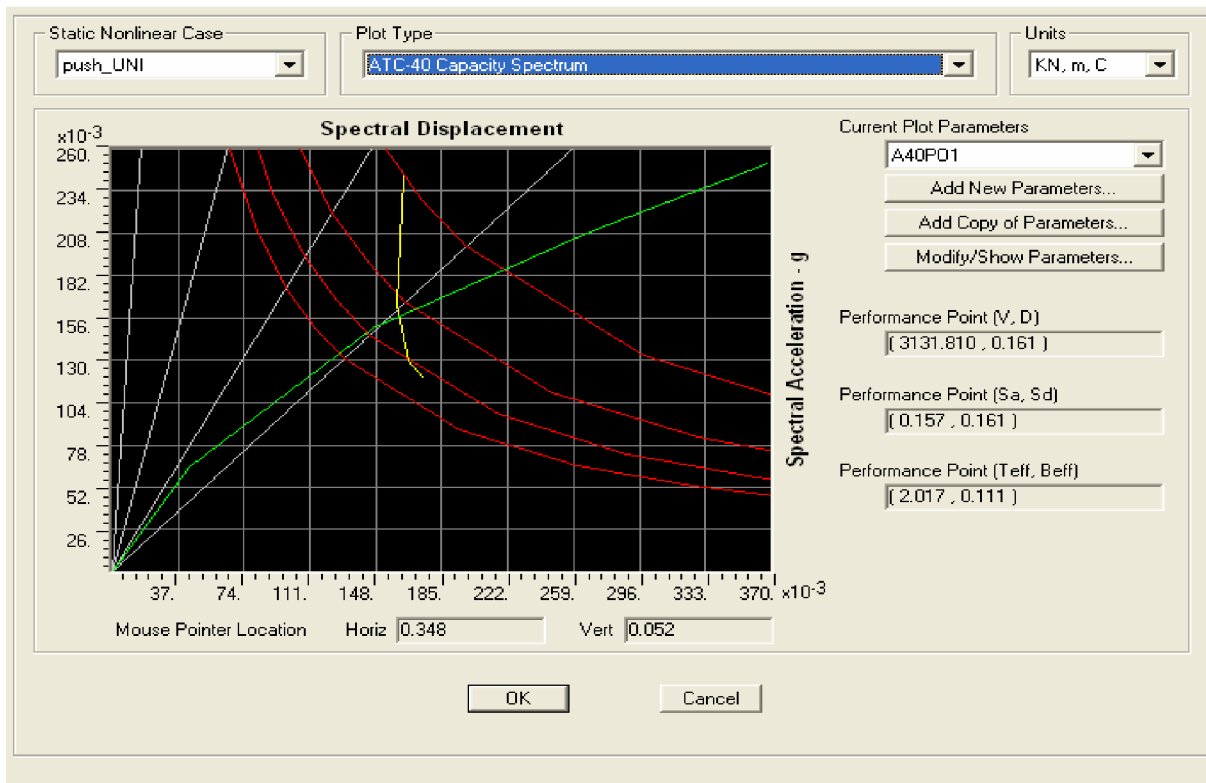
Fig.4.16 Capacity spectrum of eight storey building for Triangular Load Pattern
