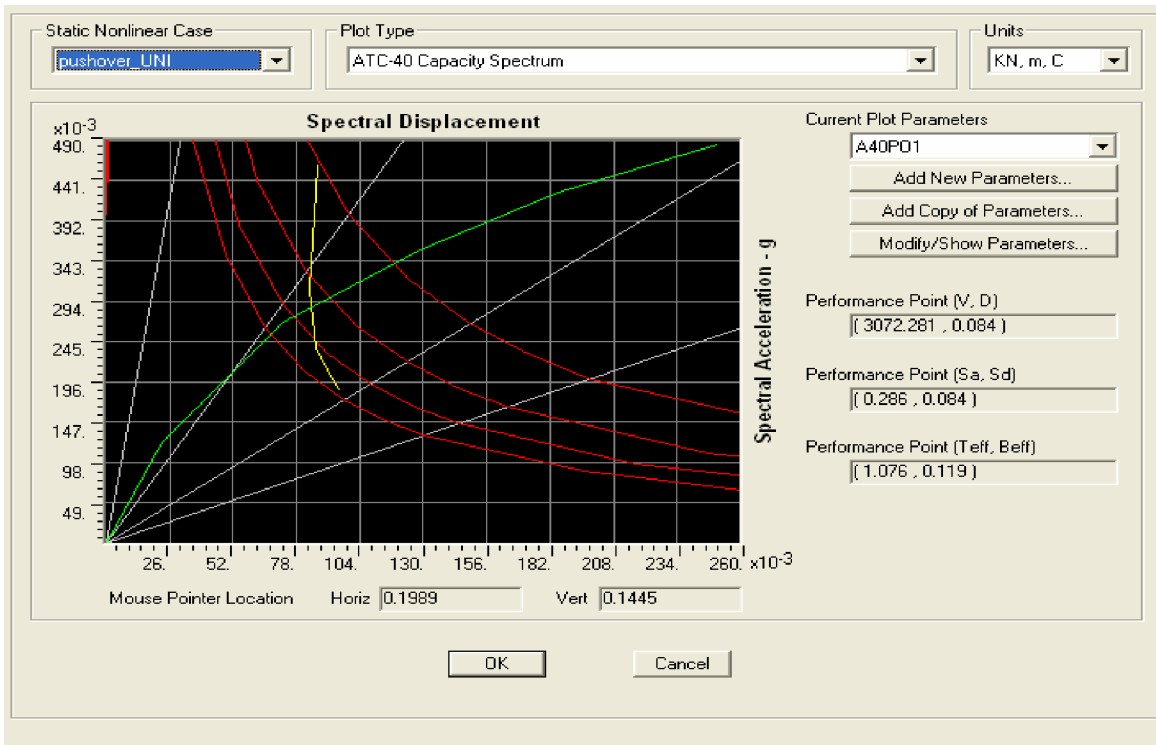
Fig.4.14 Capacity spectrum of four storey building for Uniform Load Pattern.
