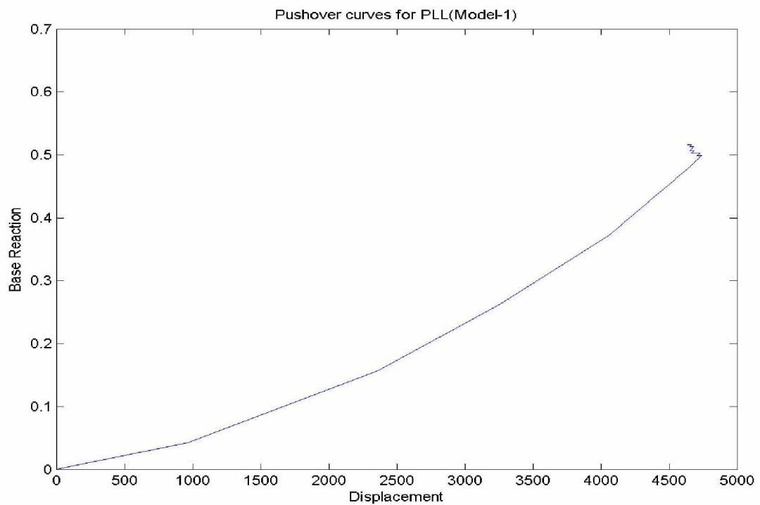
Fig 4.4 Pushover curve for parabolic lateral load pattern
