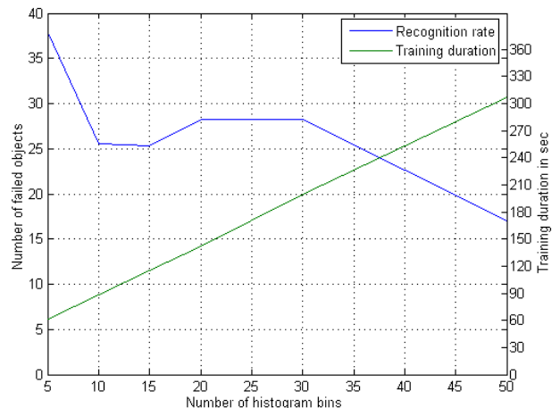
Fig. 4 Training duration vs. recognition rate for different bin sizes.
