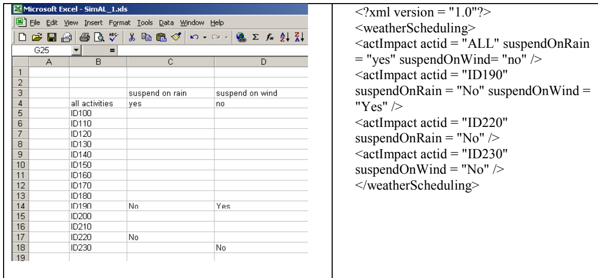
Figure 6: Encoding Domain Knowledge in XML via a Excel Spreadsheet
