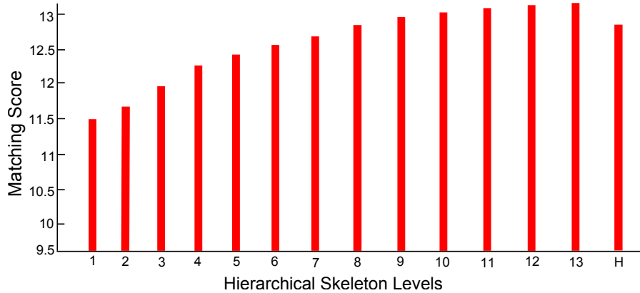
Fig. 10. Shape retrieval results using different levels of hierarchical skeletons on MPEG7 dataset. H illustrates the shape retrieval results using the perceptually complete hierarchical skeletons.
