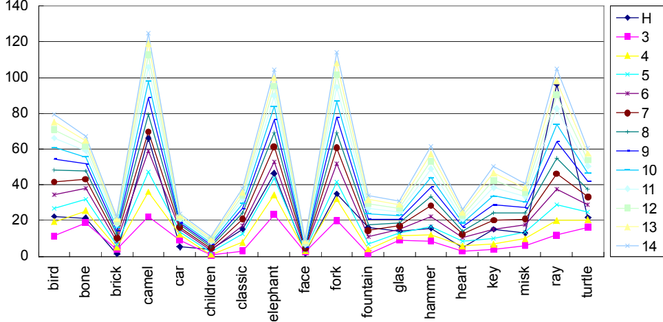
Fig. 8. Comparison of the mean dissimilarity values between skeletons in each class. Skeletons are generated by machine in Section II-A with k \in [3, 14] and human perception in Section II-B.
