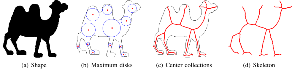
Fig. 2. An overview of the skeletonisation process with the Max-Disc method [13].
