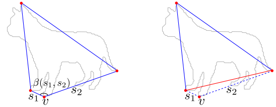
Fig. 5. Polygon simplification. As vertex v has the smallest contribution with Eq. 1, its consecutive line segments s_1, s_2 are replaced by a single line segment (red line).
