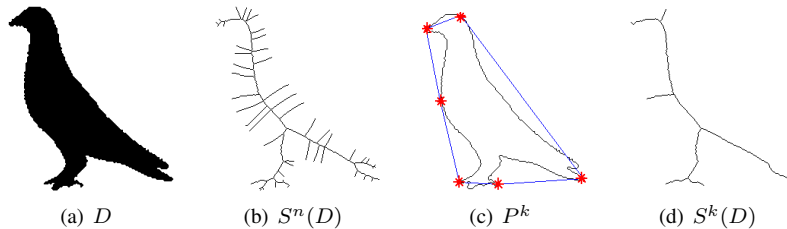
Fig. 4. Illustration of original shape D , initial skeleton S^n(D) , simplified polygon P^k and the pruned skeleton S^k(D) .
