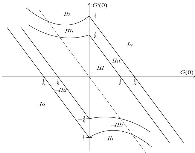
Fig. 2. The map of the self-similar solutions. The regions Ia, IIa are separated from Ib, IIb by the G'(0) axis. The infinite region III extends over all area encompassed by the stripes IIa, IIb, -IIa , -IIb , except for the origin (0,0) which corresponds to the trivial solution G = 0 . The stripe IIb asymptotically approaches the stripe -IIa , similarly IIa approaches -IIb .
