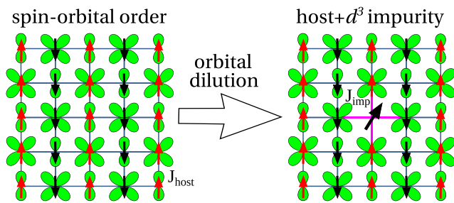
Fig. 1 Left —spin-orbital C -AF/ G -AO order found in Mott insulators with d^2 (vanadates) or d4 (ruthenates) ionic configurations. Spins S = 1 are shown by red (black) arrows and doubly occupied t_{2g} orbitals (doublons) are shown by green symbols for a and c orbitals. Right —the orbital dilution occurs after doping by a 3d^3 ion with S = 3/2 and no orbital degree of freedom. Here, a doublon site is replaced by \text{Mn}^{4+} or \text{Cr}^{3+} impurity coupled to the host by 3d - 4d bonds
