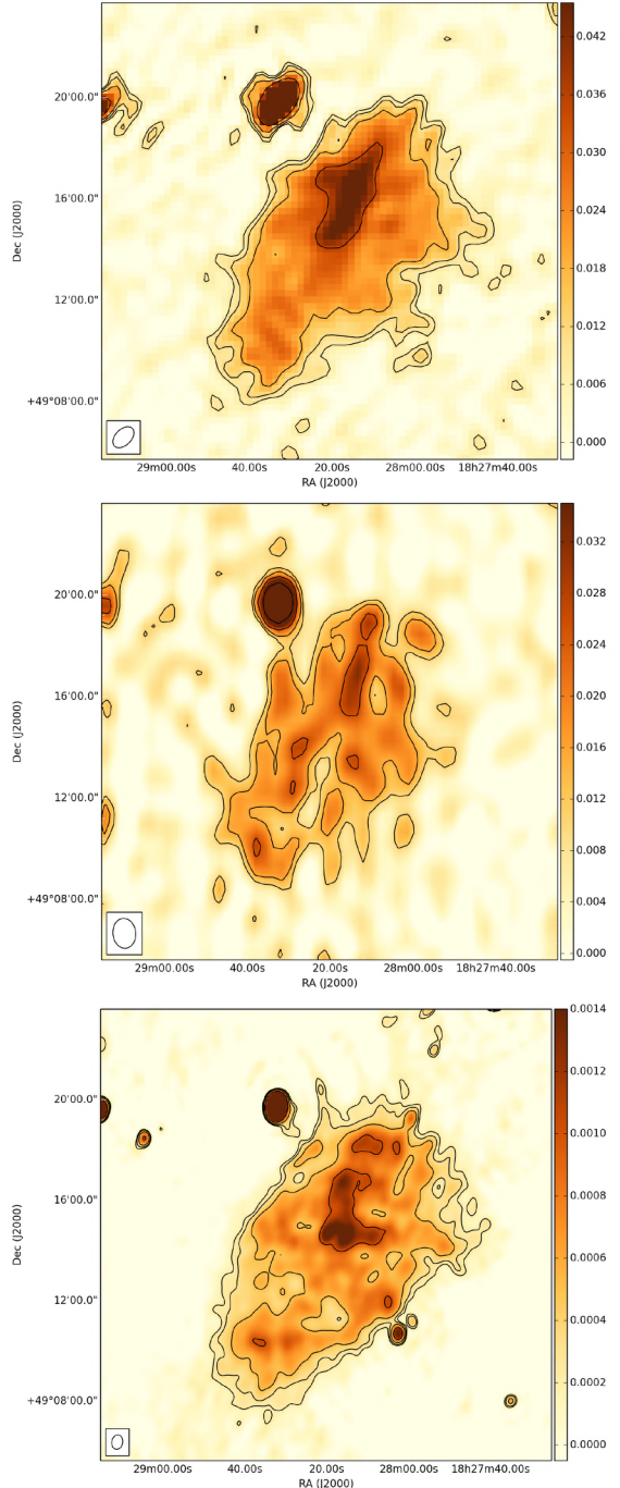
Fig. 1. Radio maps of blob1: (top panel) LOFAR 137-MHz map, levels 2, 3, 5, 10 \times \sigma (3.5 mJy \text{beam}^{-1} ); (middle panel) WENSS 327-MHz map, levels 2, 3, 5, 10 \times \sigma (5 mJy \text{beam}^{-1} ); (bottom panel) WSRT 1400-MHz map, levels: 2, 3, 5, 10 \times \sigma (0.08 mJy \text{beam}^{-1} ).
