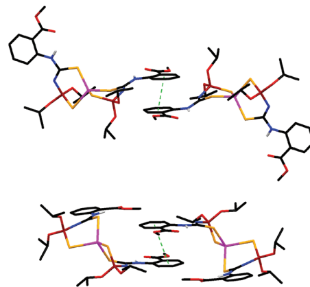
Fig. 2 Dimers formed via \pi ... \pi stacking interactions in the structures of [ZnL 2 ] (top) and [CdL 2 ] (bottom). Hydrogen atoms except NH were omitted for clarity. Colour code: C = black, H = light grey, N = blue, O = red, P = brown, S = yellow, M = magenta.
