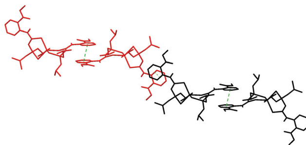
Fig. 3 1D polymeric chain formed via \pi ... \pi stacking interactions of the \pi ... \pi stacked dimers in the structure of [ZnL 2 ]. Hydrogen atoms except NH were omitted for clarity.
