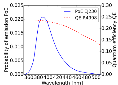
Fig. 1. Emission spectrum of the EJ230 material [15] and quantum efficiency of the R4998 photomultiplier [17].
