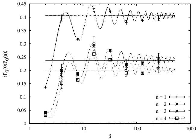
Fig. 2. Comparison of \langle P_Q^\dagger P_Q \rangle measured on a 6 \times 6 lattice (data points) with the analytic prediction of Eq. (7) and with the continuum limit given by Eq. (17) (horizontal lines).
