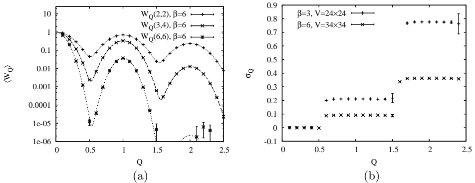
Fig. 1. Numerical data for charged Wilson loops. The Hybrid Monte Carlo algorithm was employed for the simulations, and lattices of size 24 \times 24 at \beta = 3 (48 million measurements) and 34 \times 34 at \beta = 6 (19.2 million measurements) were used. (a) Monte Carlo data for charged Wilson loops. (b) Extracted string tension \sigma_Q as a function of charge for \beta = 3 and \beta = 6 .
