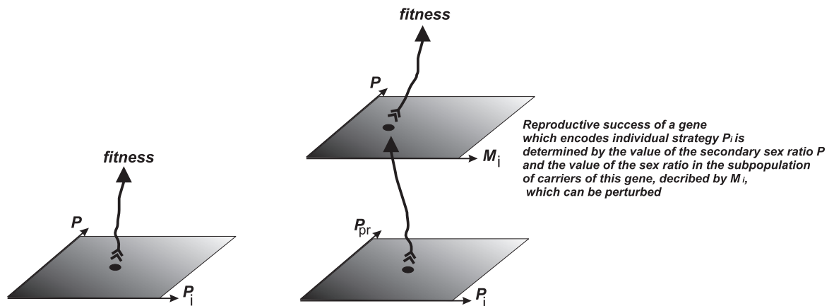
Classical Dusing-Fisher theory relies on the assumption, that fitness is unambiguously determined by the values of the individual strategy P_i and the secondary sex ratio P .
