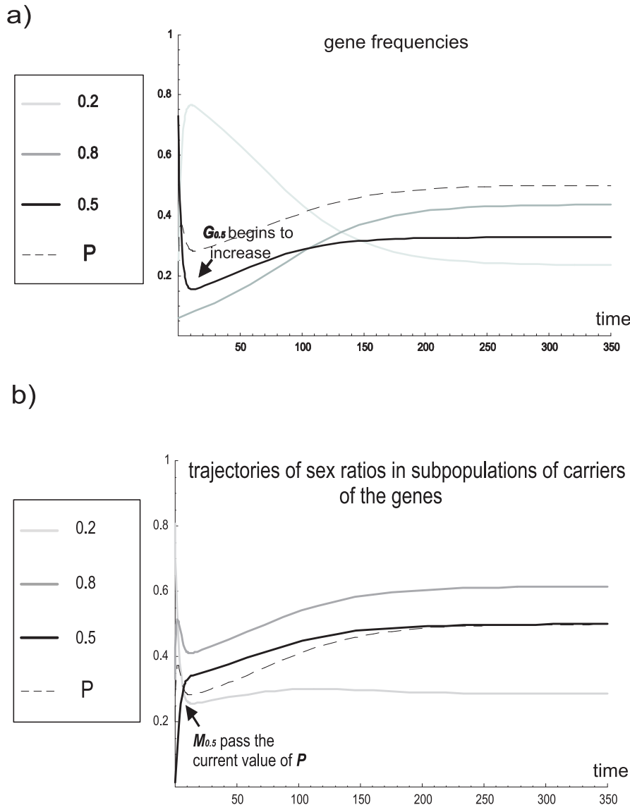
Figure 2. Trajectories of a population of individuals with strategies for sex ratios of 0.2, 0.5 and 0.8 for initial conditions. f_1 = f_2 = 0.05 , f_3 = 0.9 , m_1 = 0.85 , m_2 = 0.1 , m_3 = 0.05 . Panel a) shows the trajectories of gene frequencies G_i . Therefore, G_i increases when P < \frac{1}{2} and P < M_i or P > \frac{1}{2} and P > M_i and decreases when P < \frac{1}{2} and P > M_i or P > \frac{1}{2} and P < M_i . This mechanism is clearly shown in the trajectories of strategy 0.5. The trajectory G_{0.5} switches from a decrease to an increase when trajectory of M_{0.5} passes the trajectory of P (see panel b). Panel b) shows the respective changes of sex ratios in carrier subpopulations M_i . Note that sex ratios in carrier subpopulations rapidly converge to the values determined by the MSE phenomenon, and after that, they follow the changes of the primary sex ratio \bar{P}_{pr} that slowly converges to 0.5. The sex ratio among carriers of male biased strategies change due to the dynamics of the primary sex ratio while among female biased strategies, it converges to the neighbourhood of the value encoded by the gene. doi:10.1371/journal.pone.0060405.g002
