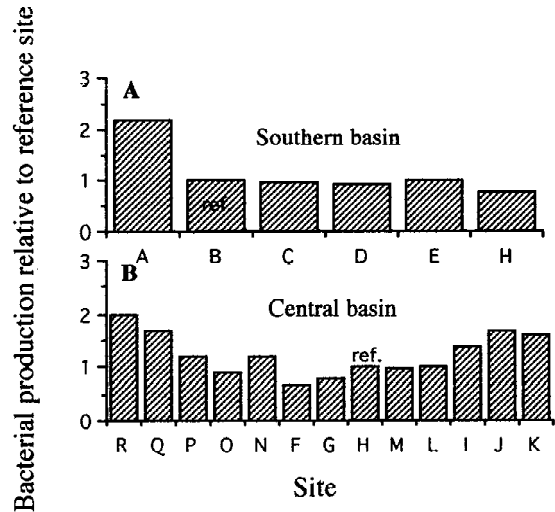
Figure 4. Bacterial production from monthly sampling (1991–1992) of transects in (a) southern basin and (b) central basin, with sampling sites arranged according to depth and position within basins (see Figure 1). The bacterial production at each sampling site is expressed as a yearly water column average value relative to a reference station, which was the regular sampling sites 1 (B) in the southern basin and 2 (H) in the central basin.
