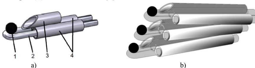
Fig. 1. Scheme of the droplet ejection device. The single droplet ejection module (a). There are: 1 – the CWSP droplet; 2 – thin nichrome wire; 3 – cutting element; 4 – metal guiding pipe. The synchronized ejection device for three fuel droplets (b) consists of three modules presented at (a).
