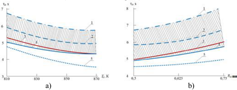
Fig. 2. The dependences (a) of the CWSP ignition delay time with oxidant flow temperature at R_d=0.5 mm and V_g=3.5 m/s. The ignition delay time changes with CWSP droplet size (b) at T_g=813 K. Curves 1, 2, 4 corresponds to ignition of the first, second and third droplets in order of ignition events. The curve 3 corresponds to ignition of the single droplet inside the chamber. The curve 5 corresponds to ignition of typical small secondary droplets segregated from one of the initial set due to collision with chamber walls.
