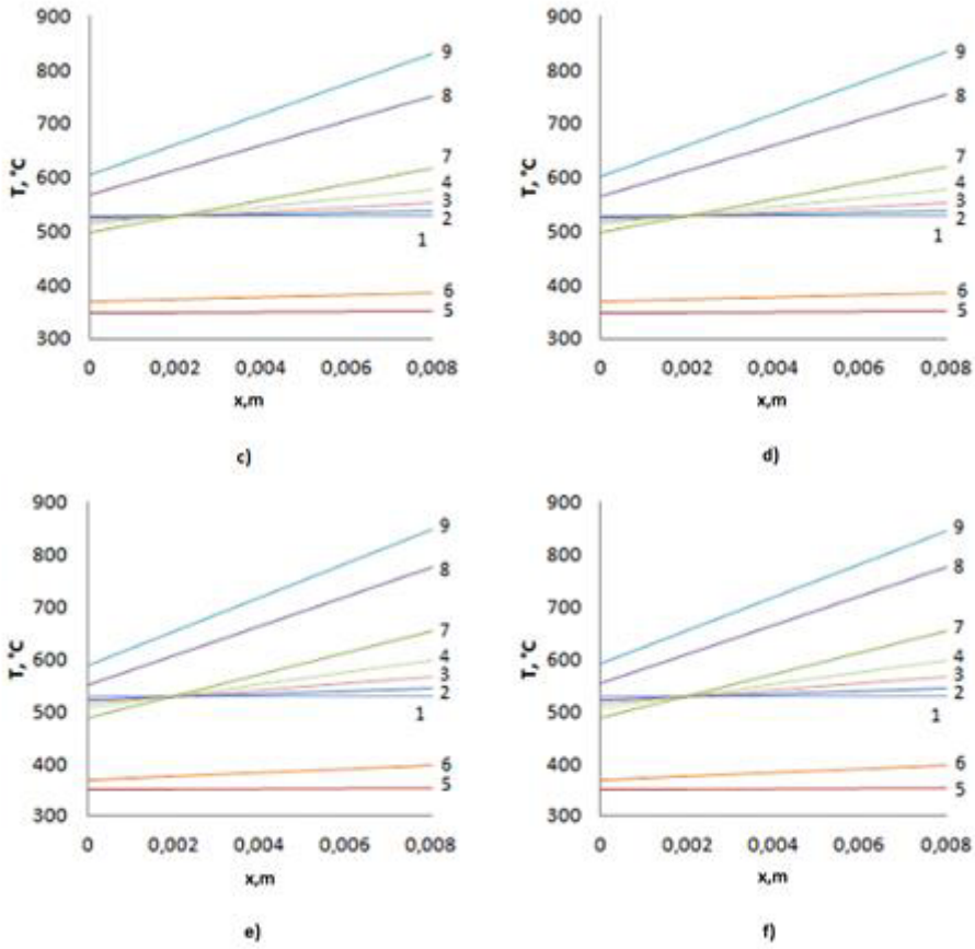
Fig. 1. Plane wall temperature distributions diagrams for steel, K: a – St.10; b – St. 20; c – 12Kh1MF; d – 15KhM; e – 12Kh18N12T; f – 1Kh18N9T.
