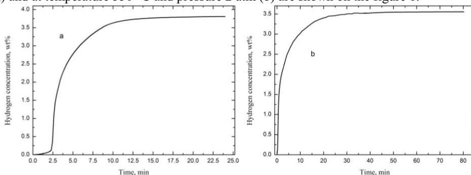
Fig. 1. Hydrogen sorption curves by titanium powder at temperature 400 °C and pressure 0.5 atm (a) and at temperature 550 °C and pressure 2 atm (b).
