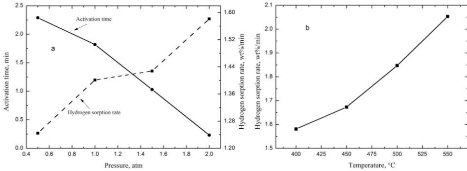
Fig. 2. The dependence of powder activation time (the solid line) and hydrogen sorption rate (the dotted line) on the pressure at constant temperature 400 °C (a) and dependence of hydrogen sorption rate on temperature at constant pressure 2 atm (b).
