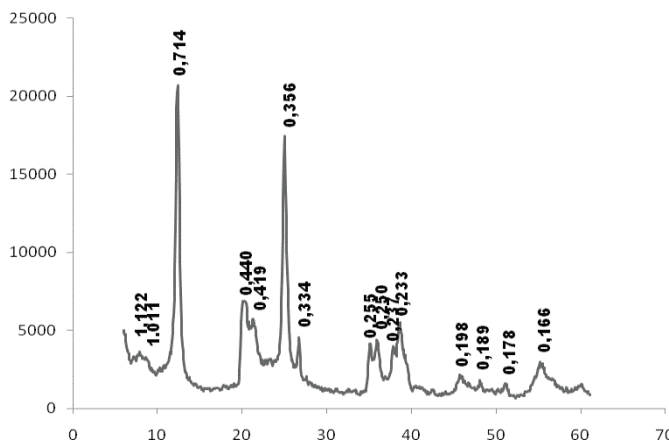
Fig. 1. X-ray diffraction pattern of Borovichy kaolin
