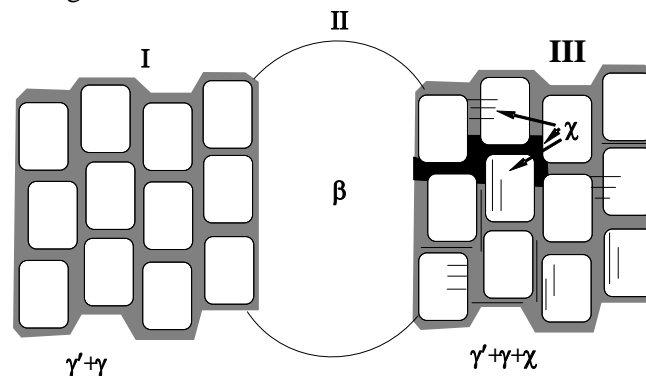
Figure 1. Schematic imagination of the structure of the alloy. Three morphologically-phase states: I - ideal structure of quazi cuboids ( \gamma'+\gamma ); II-section II of \beta -phase; III - quazi cuboids ( \gamma'+\gamma ), containing layers \chi -phase
