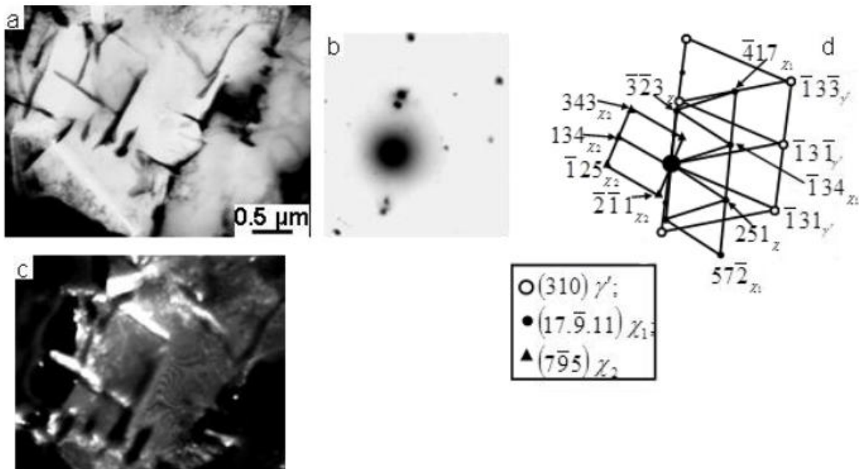
Figure 3. TEM image of structure-phase state III: a – bright-field image; b – microdiffraction patterns; c – dark-field images, obtained in reflex [\bar{3}23]_x and d - scheme indexing (b)
