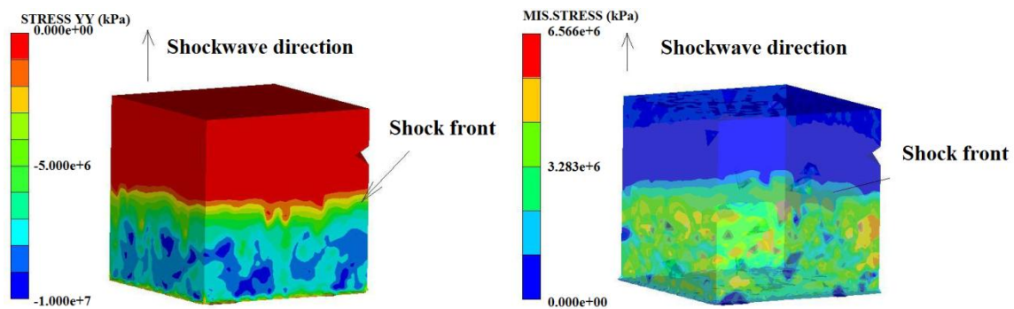
Figure 1. Distribution and strength of shear stresses during the shockwave propagation in \text{Al}_2\text{O}_3 -(15vol.%t- \text{ZrO}_2 ) composite material
