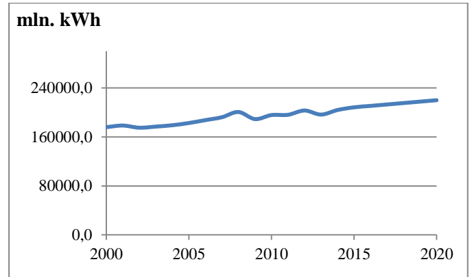
Fig.5. Population electric consumption forecasting of SFD, mln. kWh
