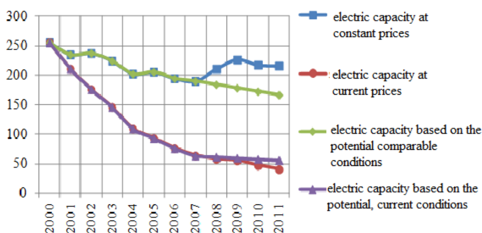
Fig.3. GRP electricity intensity in current and comparable conditions with and without the energy saving potential.
