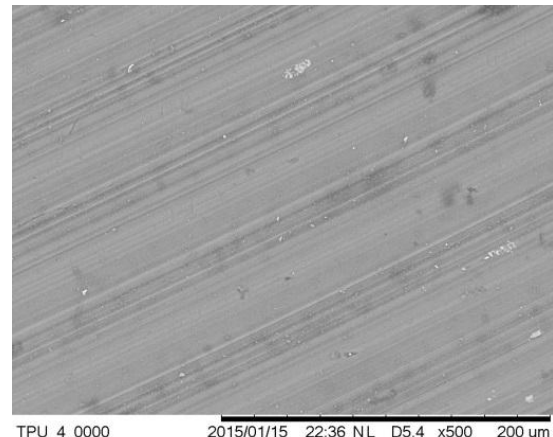
Figure 2. Microstructure of magnesium substrate ( R_a=0.51 \mu\text{m} ).
