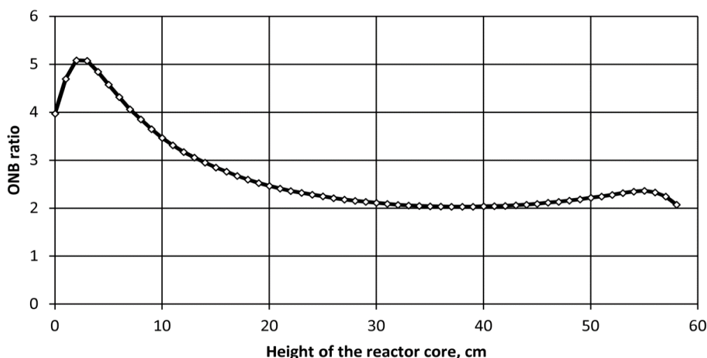
Figure 1. ONB ratio for the outer fuel element of the most stressed eight-tube fuel assembly during the first cycle at inlet coolant temperature 45 °C.
