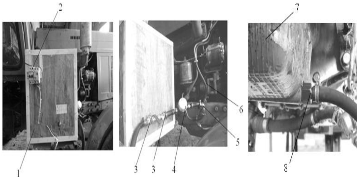
Figure 2. Pre-launch oil supply device into the lubrication system of the engine D-240: 1 - thermoinsulated hydraulic accumulator; 2 - module for the connection of the oil heater with the external network; 3 - tap; 4 - fluid meter; 5 - tee-joint; 6 - main oil passage; 7 - oil crankcase of the engine D-240; 8 - connector of the drain hole.
