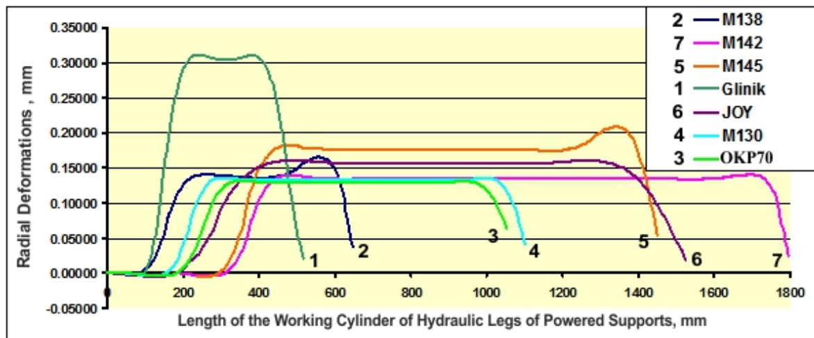
Figure 3. Radial Deformations Along the Length of the Working Cylinder of Hydraulic Legs of Powered Supports at Extension l_p=l_p^{max} and P=50 MPa
