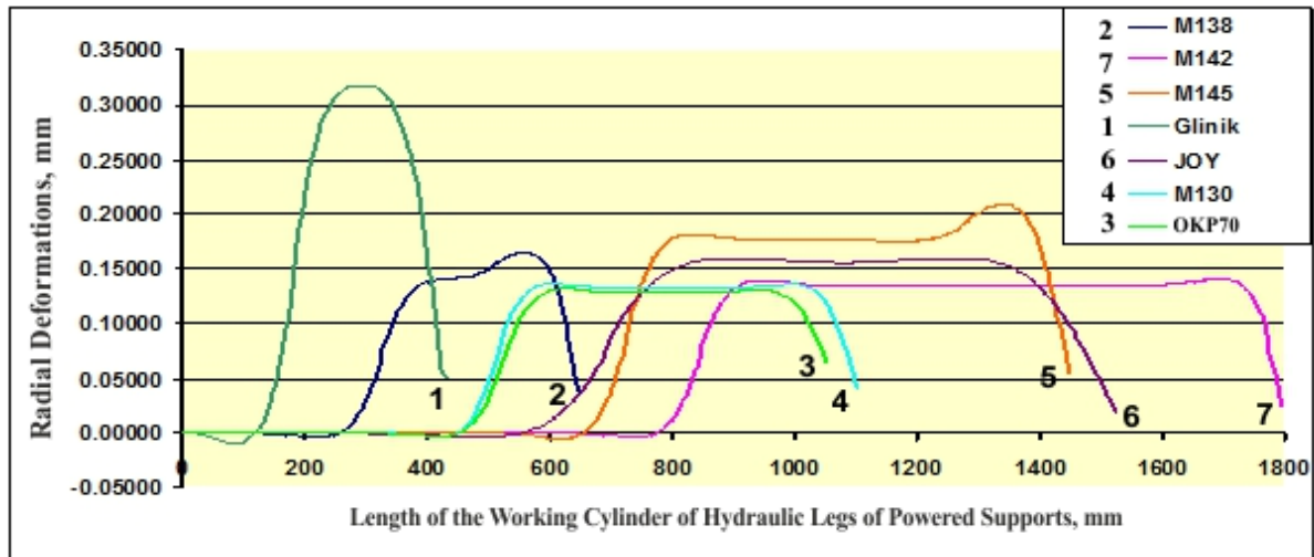
Figure 2. Radial Deformations Along the Length of the Working Cylinder of Hydraulic Legs of Powered Supports at Extension l_p=(2/3)l_p^{max} and P=50 MPa
