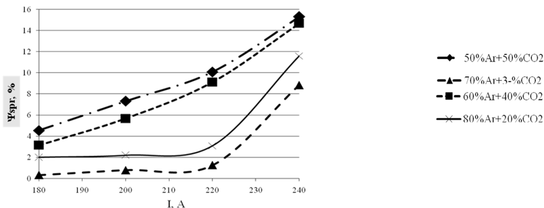
Figure 2. Dependency diagram of value of electrode metal losses by burning and spattering ( \psi_{spr} , %) of the value of arc welding current (I).
