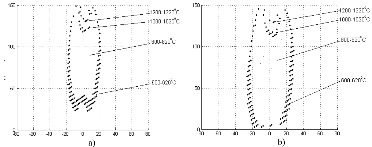
Figure 5. Experimental thermograms obtained after treatment: a) isotherm of temperature increment on the surface of weld while welding by traditional method; b) isotherm of temperature increment on the surface of weld while welded by the suggested method
