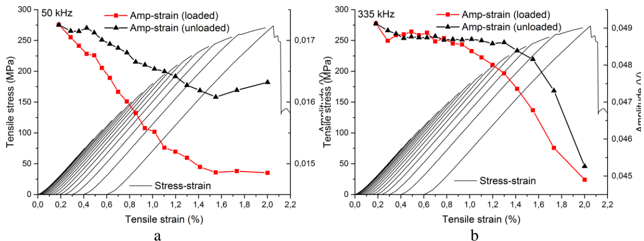
Figure 3. Combined stress-strain and amplitude-strain graphs for the step-mode tension test of the welded AA2024T3 specimen.
