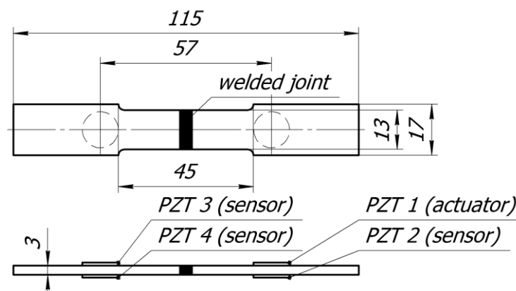
Figure 1. The drawing of the specimen, the position of the PZTs is schematically described.
