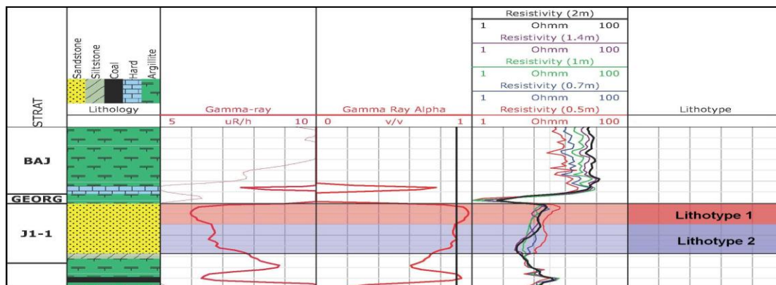
Figure 4. Well No 403 summary plot indicating lithotype classification.
