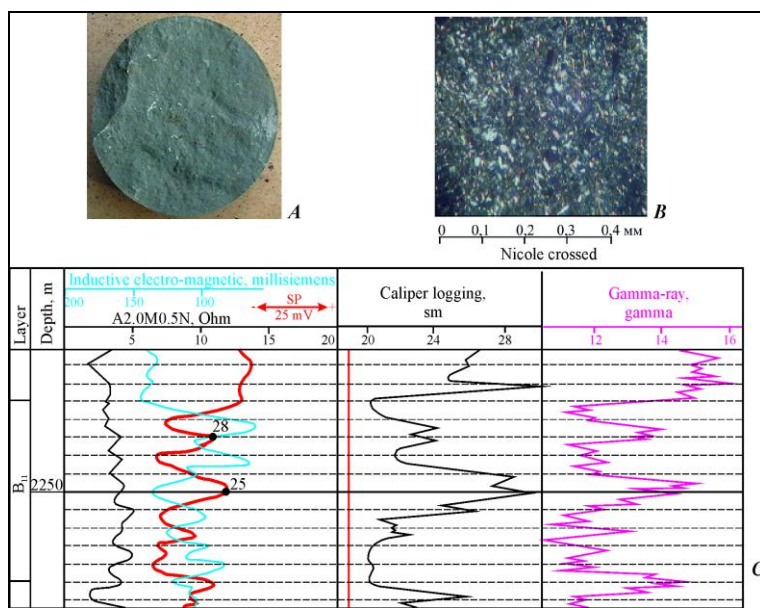
Figure 3. Structure (A), petrographic composition (B) and geophysical characteristics (C) of chlorite-hydromica clays of marine genesis:
