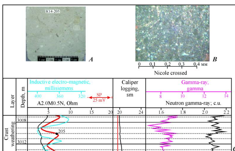
Figure 1. Structure (A), petrographic composition (B) and geophysical characteristics (C) of kaolinite clay rocks of the crust weathering: A, B, C – Well 14 Kalinovaya; depth=3010.0 m.
