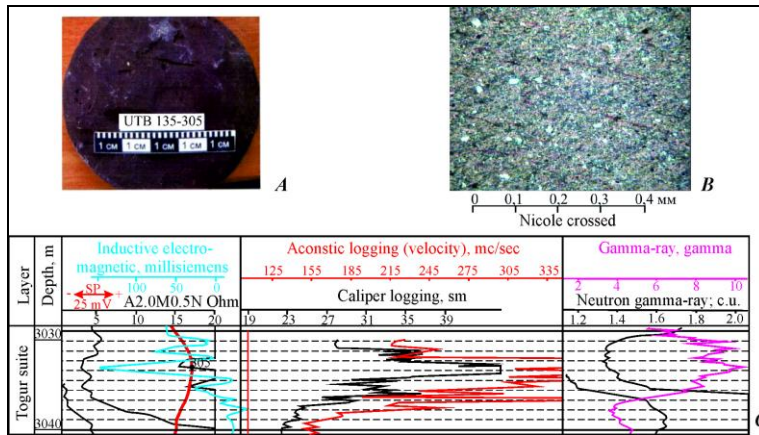
Figure 5. Structure (A), petrographic composition (B) and geophysical characteristics (C) of Togur subsuite bituminous hydromica argillite with pyrites and fine-grained quartz impurities: A, B, C – Well 135 South-Tabaganskaya; depth=3033.5 m.
