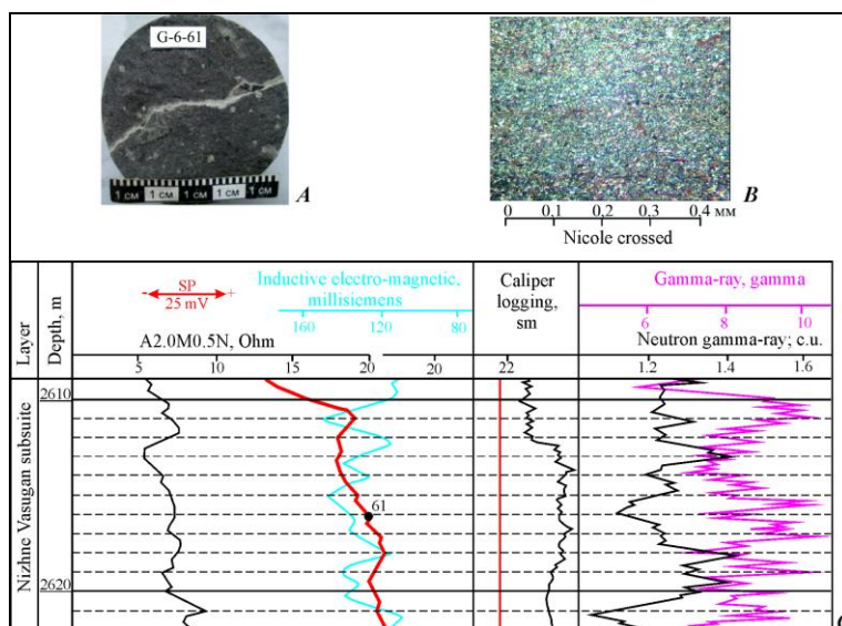
Figure 4. Structure (A), petrographic composition (B) and geophysical characteristics (C) of Nizhne-Vasugan subsuite hydromica clay rocks:
