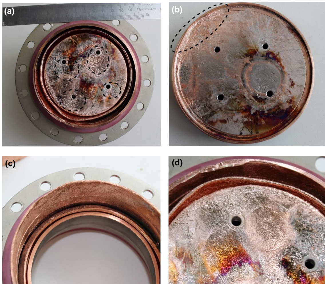
Figure 4. Internal structure of TD11-200k/25SN-P
