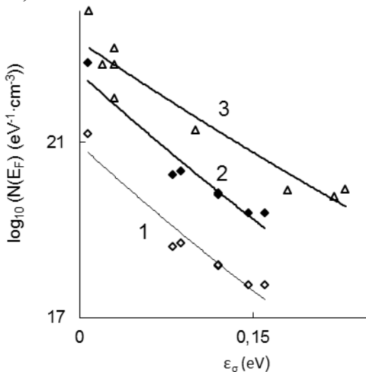
Figure 5. Interrelation between LS density and activation energy \epsilon_\sigma in the deposited films (1, 2) and according to [7] (3). Attenuation constant \alpha=5.7 \cdot 10^6 (1) and 2 \cdot 10^7 \text{ cm}^{-1} (2).
