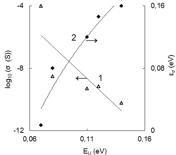
Figure 6. Interrelation between conductivity \sigma Urbach energy E_U (1) and activation energy \epsilon_\sigma and E_U (2) in the deposited films. The values E_U are calculated within the interval h\nu=1.15-1.3 eV.
