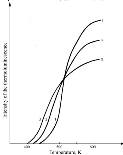
Figure 1. Thermally-stimulated luminescence of the undyed polymer produced under different curing temperatures
