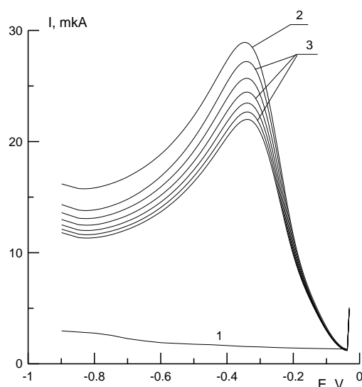
Figure 1. Voltammograms of the ER O_2 current in phosphate buffer (0.025M, pH 6.86) on the MFE without (2) and with 10^{-4} g/ml of vaccinium myrtillis aqueous extract in the solution (3), the residual current of the supporting electrolyte in the absence of O_2 and the substance in the solution (1). Potential scan rate is -40 mv / s.
