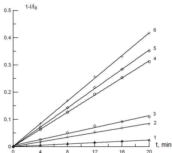
Figure 2. The linear part of the relative change of the limiting current of ER O_2 on the time of the process in the presence of 10^{-4} g/ml of vaccinium myrtillis extracts: water (1), 40% (6) 70% (4) and 95% (5) ethanol; dihydroquercetin (2), ascorbic acid (3).
