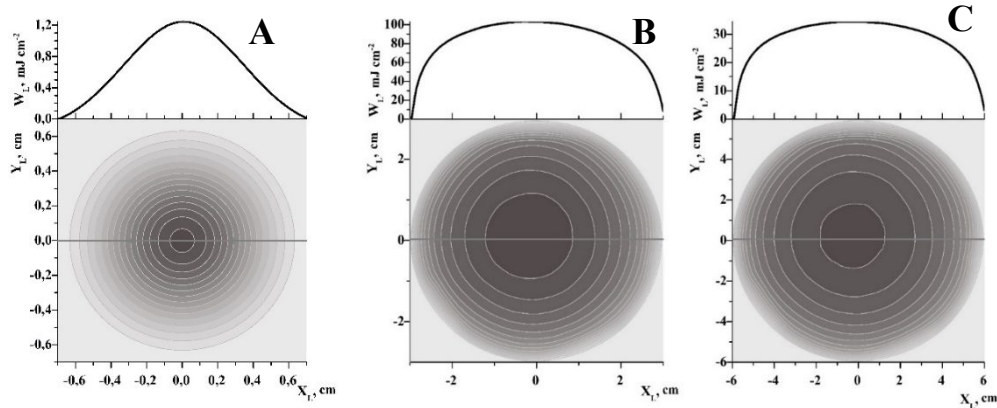
Fig. 3 Transverse distribution of laser fluence: A – Input window, B - 31 mirror. C – Output window.
