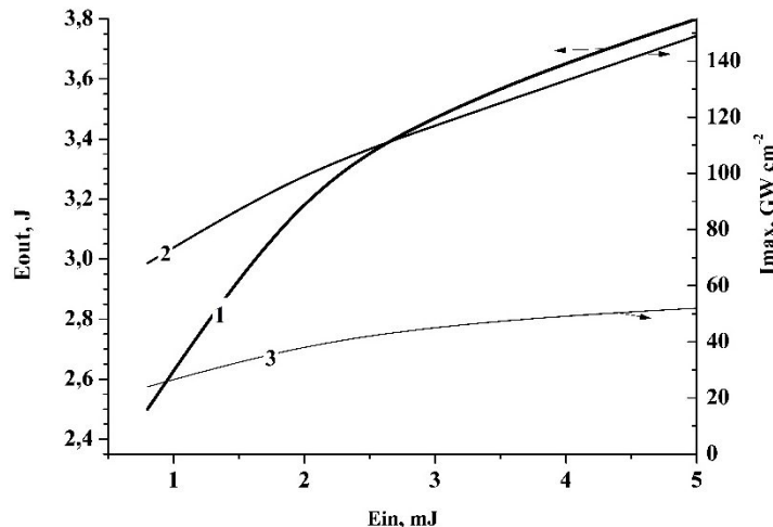
Fig 5. Laser radiation energy E_{out} -1, and maximum intensity I_{max} (mirror 31) - 2, I_{max} (output window 33) -3 as a functions of start pulse energy.
