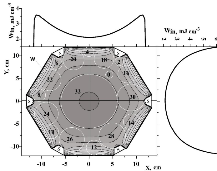
Fig. 1 Distribution of absorbed energy density in the cross section of the amplifier. Circles - mirrors. The numbers in the circle - the numbers of mirrors. S - Ribs. W - Windows to input pumping radiation.
