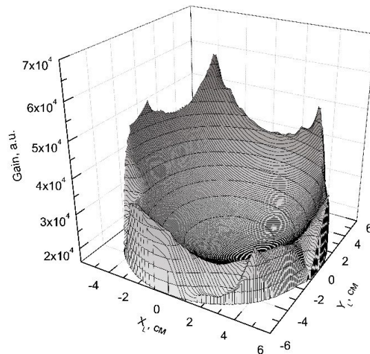
Fig. 2 Amplification in small signal gain mode. E_{SP} = 10^{-7} \text{ J}
