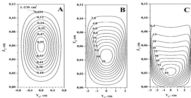
Fig.4 Distribution of the laser radiation intensity in the Y_L Z_L plane of the beam in various points of the amplifier: A - 1 pass through amplifier (mirror 1), B - 20 of passages through amplifier (mirror 20), C - 31 of passes through amplifier (mirror 31).
