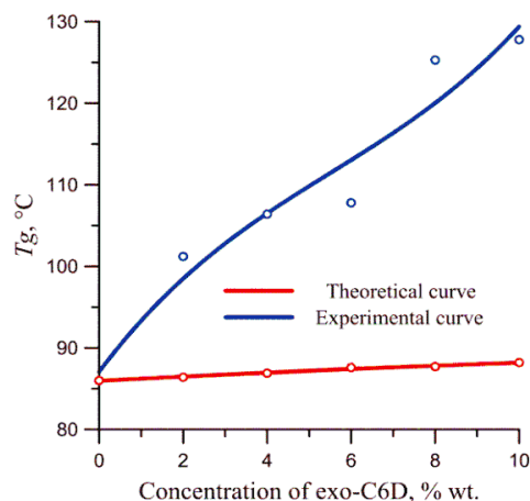
Fig. 4. Influence of concentration of exo-C6D on glass transition temperature of the polymer based PDME.
