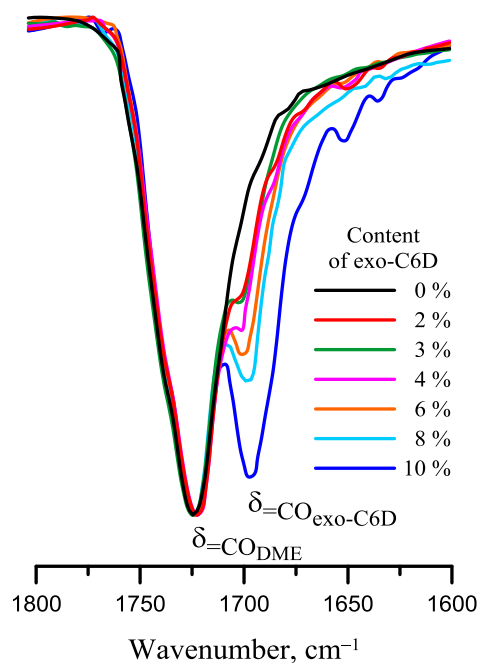
Fig. 3. IR-spectra of polymers.
