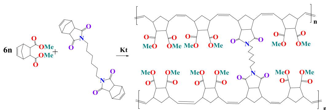
Fig. 1. Copolymerization scheme of DME and exo-C6D.
