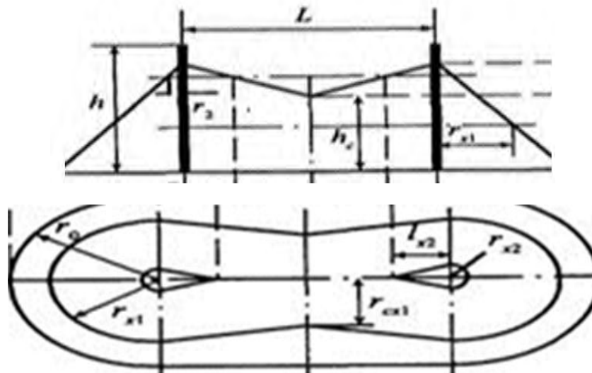
Fig. 1. Protection zone dual lightning rod
