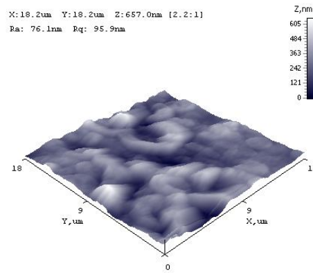
Figure 2. AFM image of the Fe-Al coating surface.
