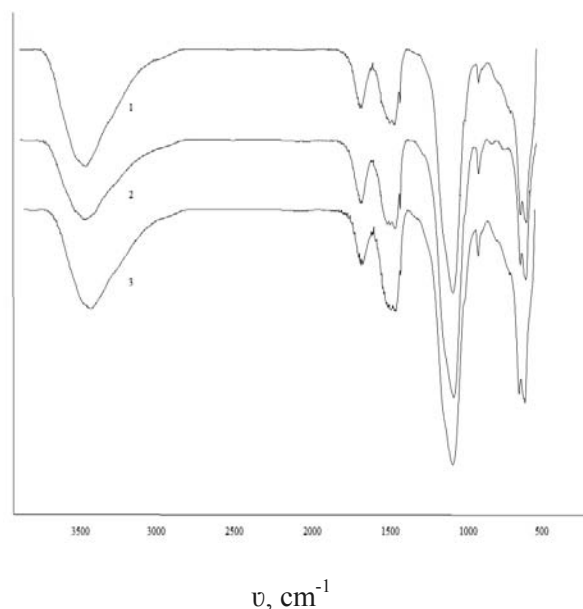
Figure 2. IR spectra for hydroxyapatite samples modified by: 1 is Na 2 SiO 3 C Si init. 0.5%; 2 and 3 are TEX C Si init. 0.5 and 2.5%.
