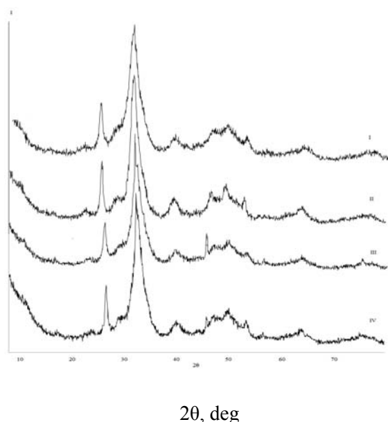
Figure 1. The diffraction patterns for hydroxyapatite samples modified by Na 2 SiO 3 : I is C Si init. 0.5%; II is C Si init. 2.5%; TEX: III is C init. 0.5%; IV is C Si Si init. 2.5%.
