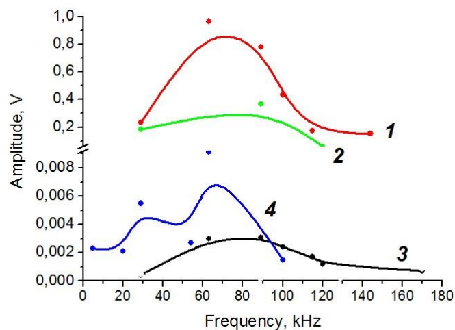
Figure 4. Dependences for the amplitude of EMS spectral components in excitation by the acoustic pulse of 10 \mu s duration for ore samples.
