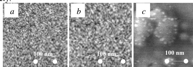
Figure 1. SEM images of the surface implanted with ^{16}O^{3+} (a), ^{40}Ar^{8+} (b) and ^{84}Kr^{15+} (c) ions.
