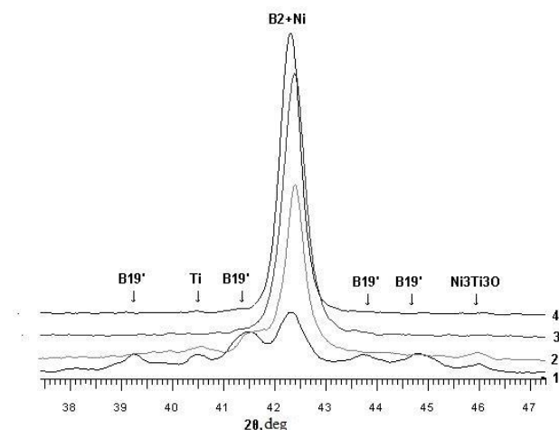
Figure 2. Parts of diffraction patterns for Ni-Ti alloy before (curve 1) and after ^{16}\text{O}^{3+} ion implantation (curve 2), ^{40}\text{Ar}^{8+} ion implantation (curve 3) and ^{84}\text{Kr}^{15+} ion implantation (curve 4).
