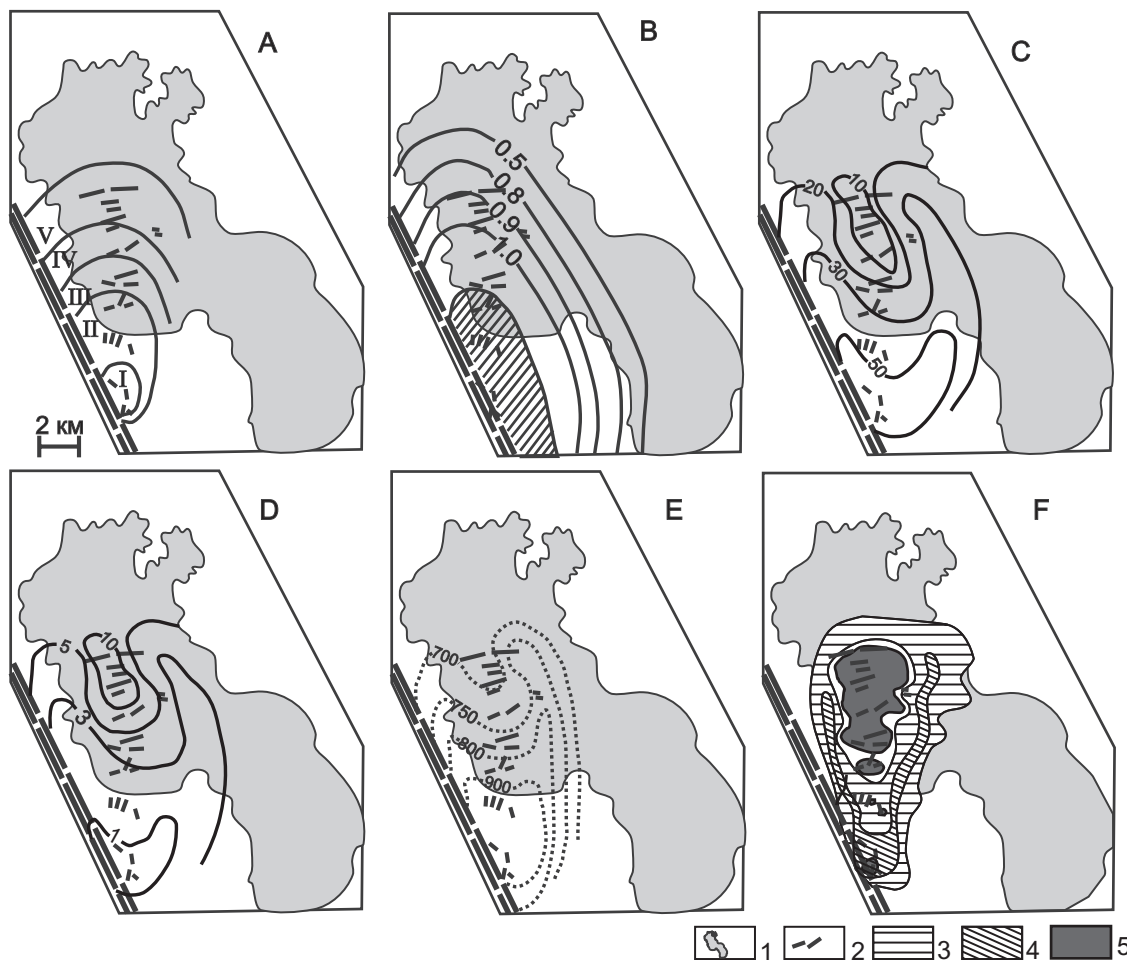
Fig. 3. The lateral zonation of the Central ore field (Kuznetsk Ala Tau): 1) the contour of granodiorite massif; 2) the basic gold-bearing veins; A) mineral zones of the ore field (on typomorphing minerals): I) tourmaline; II) scheelite; III) molybdenite – chalcopyrite; IV) galenite – sphalerite; V) arsenopyrite; B) degree of triclinicity of kalispar from zones of kalispar-epidote – chlorite metasomatites (the development area of a latticed microcline is shaded); C) the share of pyrites with electron type of conductivity (in %) in gold-bearing quartz-sulphidic veins; D) intensity of natural thermo luminescence of vein quartz (in standard units); E) grade of native gold in quartz-sulphidic veins; F) storage sites of geochemical associations: 3) V, Ti, Ba, Zr, Sr; 4) Ni, Co, Cr; 5) Au, Cu, Zn, Pb, Ag, As
