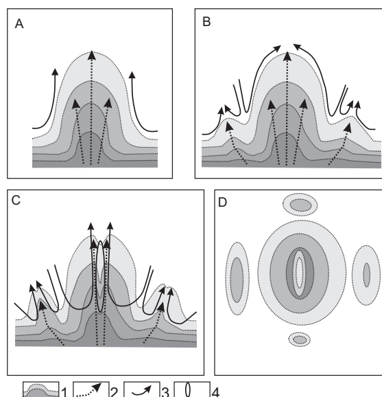
Fig. 1. Model of temperature evolution of endogenous thermo-fluidic systems: 1) isolines of fluid temperature distributions; 2) directions of movement of a endogenous fluid; 3) ways of convective currents of local solutions; 4) areas of temperature and pressure fall, including steam zones; A, B, C) stages of temperature evolution of hydrothermal system (cuts in a vertical plane); D) horizontal section of system at a final stage of ore deposition
