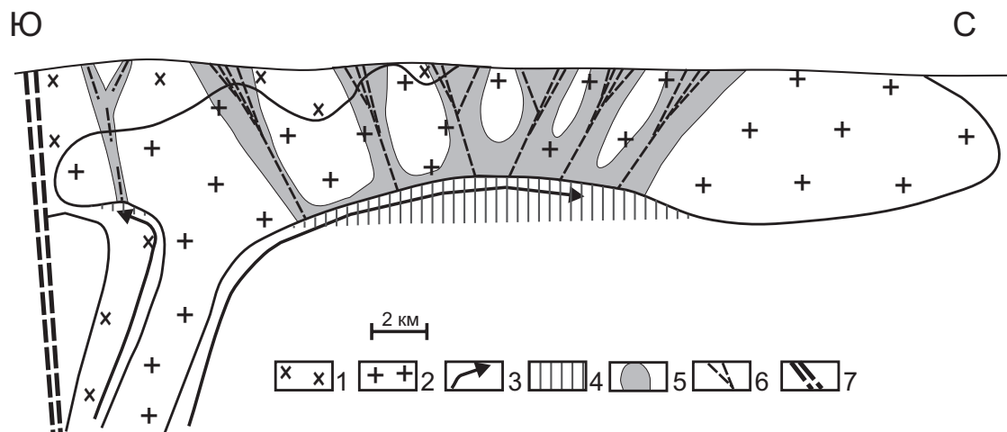
Fig. 4. The schematic cut of the Central ore field (Kuznetsk Ala Tau): 1) horned and uralitized gabbro-diorites (metadiorites); 2) granodiorites, tonalites, quartzitic diorites; 3) stream of a deep fluid; 4) storage field of a gaseous fluid under a cover of cooling down intrusive; 5) area preore metasomatites; 6) the cracks controlling and containing of ores; 7) the Kuznetsk Ala Tau deep break
