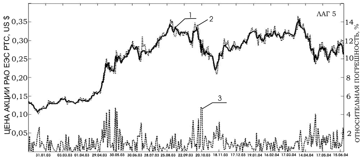
Fig. 3. Comparison of historical and model quotation values of RAO UES RTS shares from January 04, 2003 to June 30, 2004: 1) time series of historical data, 2) time series, calculated by STS-GARCH(1,1) with lag 5, 3) relative error, %
