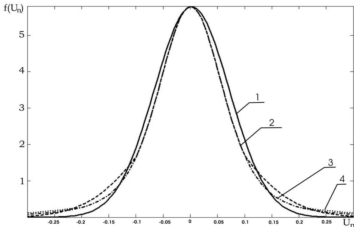
Fig. 2. Densities of STS-distribution at \alpha=1,5 , \beta=0,1135 , c=0,05 , \mu=0,00191 and density function of normal distribution with mathematical expectation \mu and variance 0,00476 : 1) density of the normal probabilistic law; 2) density of STS at a=-0,1 , b=0,1 , \rho_1=\rho_2=0,105 ; 3) density of STS at a=-0,2 , b=0,2 , \rho_1=\rho_2=0,031 ; 4) density of STS at a=-0,3 , b=0,3 , \rho_1=\rho_2=0,015
