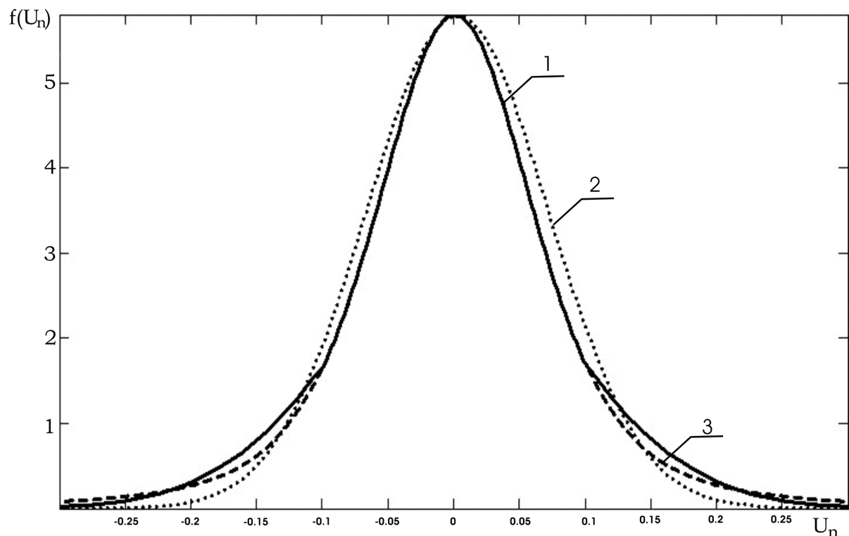
Fig. 1. Densities of normal, \alpha -stable and STS-distributions at a=-0,1, b=0,1 ( p_1=p_2=0,105 ), \alpha=1,5, \beta=0,1135, c=0,05, \mu=0,00191 : 1) density of STS-distribution; 2) density of normal distribution with mathematical expectation \mu=0,00191 and variance 0,004761 ; 3) density of \alpha -stable distribution
