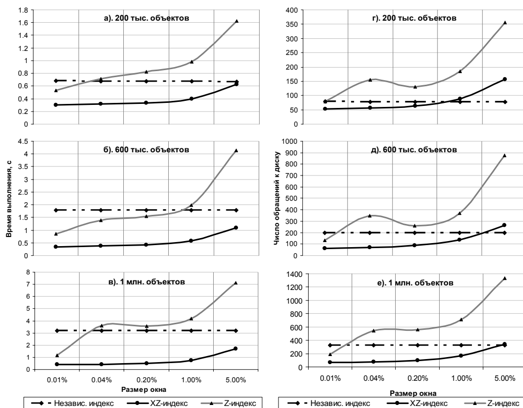
Fig. 2. Results of experiment (at the left – measurements of time, on the right – measurements of number of disk operations)
