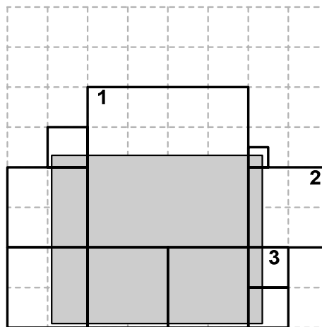
Fig. 1. Optimal splitting, N_{\max}=10
