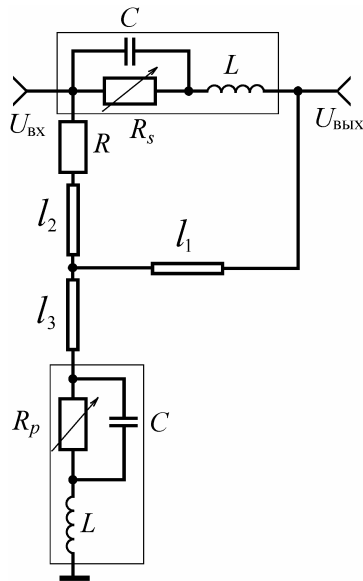
Fig. 2. DVS model
