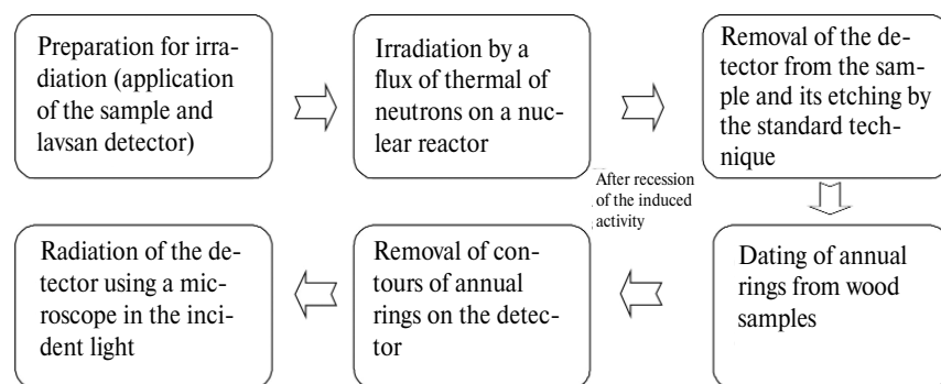
Fig. 1. The scheme of works at radiography of wood samples
