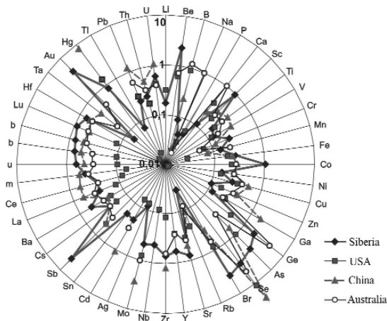
Fig. 1. Graph of element distribution in Siberian coals normed to average of the Earth's crust
