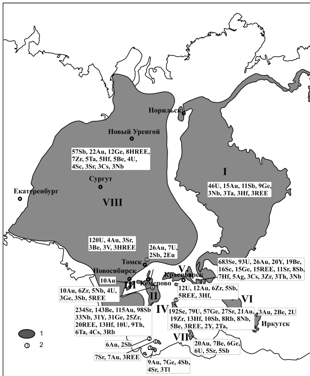
Fig. 3. Map of rare-metal specialization of Siberian coal. 1 – Coal basins: I) Tunguskiy; II) Kuznetskiy; III) Gorlovskiy; IV) Minusinskiy; V) Kansko-Achinskiy; VI) Irkutskiy; VII) Ulugkhemskiy; VIII) West-Siberian; 2 – coal fields.
