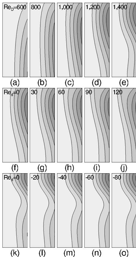
FIG. 7. Plots of circulation ( \Gamma = u_\theta r ) for various cases. Control disk is stationary and (a) Re_D = 600 , (b) 800, (c) 1000, (d) 1200, and (e) 1400. Flow at Re_D = 1200 and the corotating control disk speed varied, (f) Re_d = 0 , (g) 30, (h) 60, (i) 90, and (j) 120. Flow at Re_D = 1835 and the counter-rotating control disk speed varied, (k) Re_d = 0 , (l) -20 , (m) -40 , (n) -60 , and (o) -80 . The contours are at intervals of \Gamma / (\omega_D R^2) = 0.005 starting from 0 at the axis.
