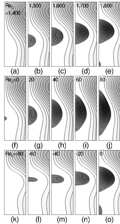
FIG. 11. Plots of stream function for various cases. Control disk stationary and (a) Re_D=1400 , (b) 1500, (c) 1600, (d) 1700, and (e) 1800. Flow at Re_D=1441 and the corotating control disk varied, (f) Re_d=0 , (g) 20, (h) 40, (i) 60, and (j) 80. Flow at Re_D=1835 and the counter-rotating control disk varied, (k) Re_d=-80 , (l) -60 , (m) -40 , (n) -20 , and (o) 0. The lighter/darker shades represent flow in the anticlockwise/clockwise direction and contoured at intervals of \Phi/(\omega_D R^2) = 1 \times 10^{-3}/1.5 \times 10^{-5} .
