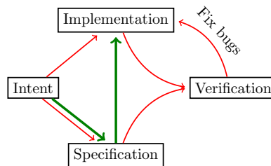
Fig. 1: Comparison of the verification (→) and synthesis (→) workflows
