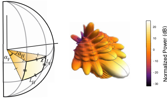
Fig. 13. Illustration of the 3D antenna radiation pattern models: right – realistic 15 \times 4 pattern obtained using the algorithm in 3GPP TR 37.977; left – 3D HPBW approximation by following [104].
