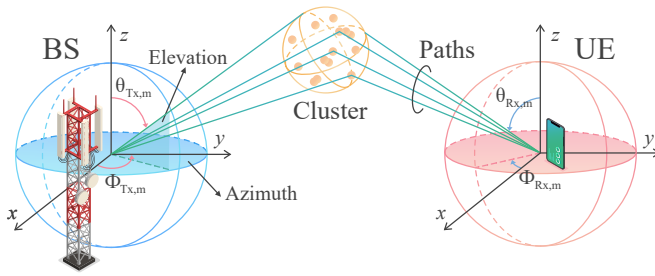
Fig. 6. Illustration of the 3D cluster-based propagation model: a number of paths between BS and UE are available each characterized with its own delay and power profiles [57].
