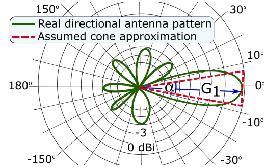
(a) 2D cone antenna model
