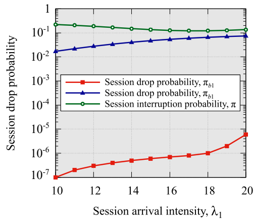
Fig. 24. Performance metrics for prioritized service at BSs: enforcing pre-emptive priority at the mmWave/NR air interface efficiently isolates higher priority traffic, e.g., URLLC, from the lower priority one, e.g., eMBB.
