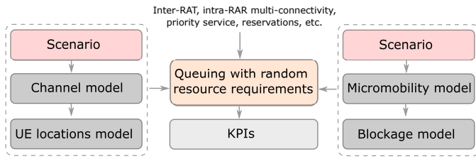
Fig. 16. Illustration of the general structure of the framework for assessing KPIs of the non-elastic/adaptive traffic in mmWave/THz RATs: the core part is the queuing model representing the process of session service at mmWave/THz BSs; the rest of the model are combined to provided abstraction of the radio part specifics.
