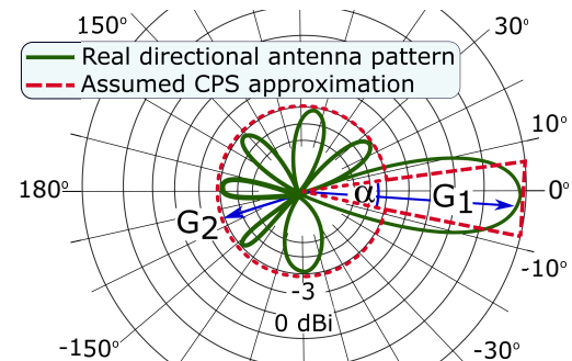
(b) 2D cone-plus-sphere model
