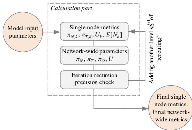
Fig. 21. Iterative algorithm for calculating performance metrics: at each stage the flow variables between BSs are updated the the difference in performance metrics at the current and previous iteration is assessed to decide on the convergence [77].
