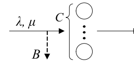
Fig. 3. Erlang's loss model – M/M/C/C queuing system: exponential arrival and service processes with intensities \lambda and \mu , finite number of servers C representing currently served sessions.
