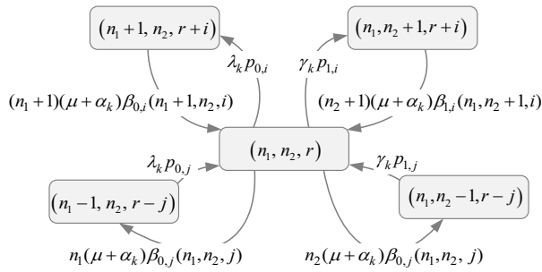
Fig. 22. Typical set of states and associated transition intensities for model representing session service process with multicconnectivity and resource reservation [77].
