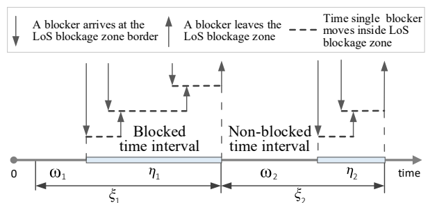
Fig. 10. Renewal process associated with the LoS blockage: blocked period is initiated by the arrival of a blocker to the LoS blockage zone and terminated when the last blocker leaves the LoS blockage zone empty; then, the non-blocked period is initiated forming a renewal process [24].
