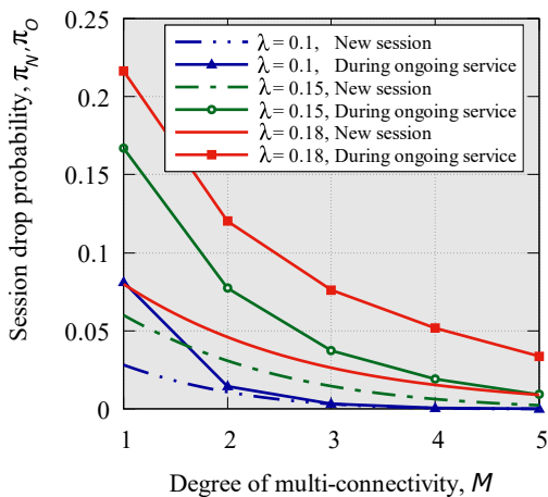
Fig. 23. New and ongoing session drop probabilities: increasing the number of mmWave/THz BS accessible for UE drastically improves service reliability including both new and ongoing session drop probability [77].
