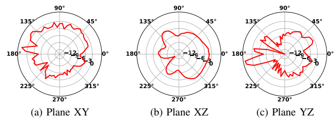
Fig. 11. Radiation pattern of Raspberry Pi 3B+ antenna plotted from anechoic chamber measurement data [61]. It is a PCB antenna designed by Proant AB present in many IoT devices operating in the 2.4GHz band.
