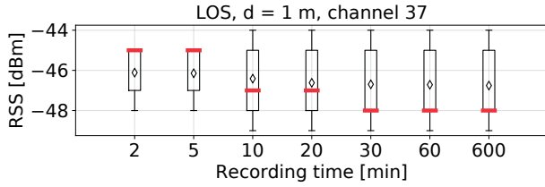
Fig. 6. The effect of the time evolution on the RSS distribution in LOS on a single channel (37), recorded at UPB.
