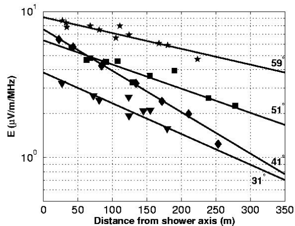
Figure 7. Electric field profiles on a logarithmic scale for a set of radio EAS events recorded on CODALEMA. The measured amplitude in \mu\text{V}/\text{m}/\text{MHz} is plotted versus the distance from the antenna to the shower axis (in meters). The associated reconstructed zenith angle is indicated on each plot.
